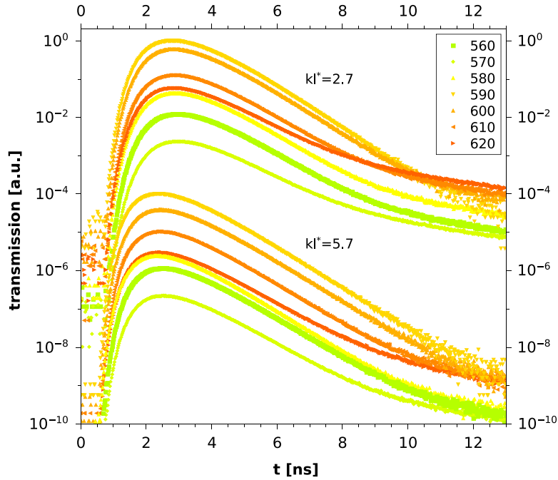
Figure 2. Time of flight distributions for fixed incident wavelength \lambda_{\text{inc}} = 590 nm ( I_0 \approx 1 GW m ^{-2} ) at different detected spectral shifts as indicated by the central wavelength of the bandpass filter \lambda_{\text{BP}} for sample R700, ( kl^* = 2.7 , L = 0.93 mm) and sample R104AA ( kl^* = 5.7 , L = 0.94 mm). The latter data are down-shifted by 4 decades for clarity.
