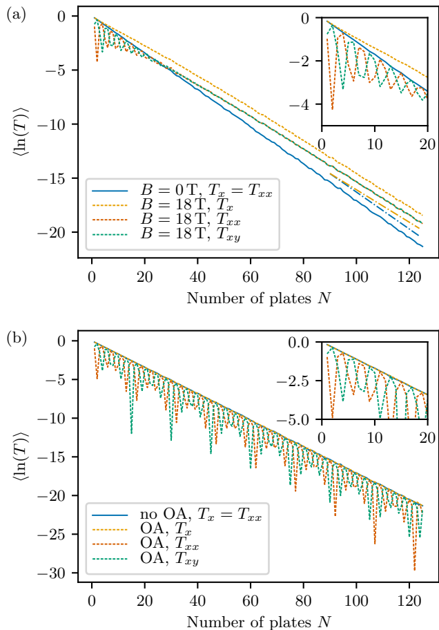
Figure 3. Average of the logarithm of T_x , T_{xx} and T_{xy} without and with (a) Faraday rotation or (b) optical activity for the same rotation angle of 48^\circ for a single passage through a single plate. This corresponds to a circular birefringence \Delta n = 4.72 \cdot 10^{-5} for FR in SF57 at B = 18\text{T} and at the average thickness of the plates.
