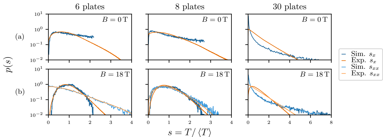
Figure 7. Histograms of the normalized transmitted intensity s = T/\langle T \rangle without (upper row, (a)) and with (lower row, (b)), B = 18 T external magnetic field for N = 6, 8 and 30 plates. Simulation data are traced in blue and experimental data in orange.
