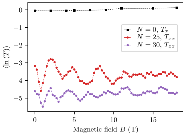
Figure 13. Experimental data of the mean logarithmic relative transmission as a function of the magnetic field B for N = 0 , 25 and 30 plates.
