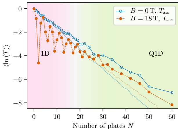
Figure 8. Experimental data of the mean logarithmic relative transmission as a function of the number of plates N at B = 0\text{ T} and 18\text{ T} . Data are measured with a polarizer at the output. The light curves are the simulation results (same data as in Fig. 3(a)).
