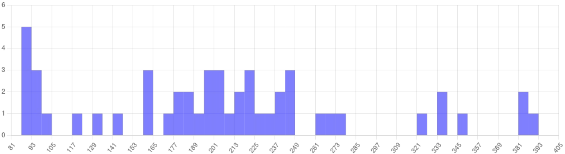
4-Lepton Events
