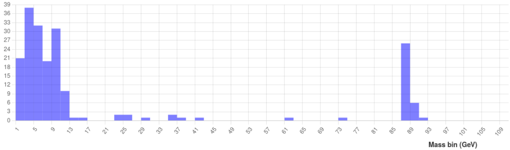
2-Lepton Events
